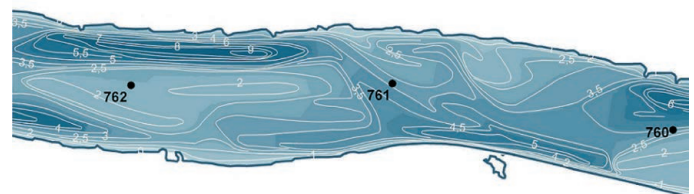
Fig. 6. Bathymetric plan of the straight channel of the Vistula (Wisła) on the Solec Kujawski section, at 760–762 km, with characteristic alternating current, regulated in the 19th century
