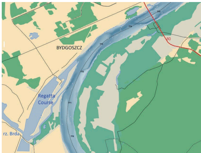
Fig. 7. Bathymetric plan of the pseudo-meander channel of the Vistula (Wisła) at the Gorge at Fordon on 770–773 km, regulated in the 19th century
